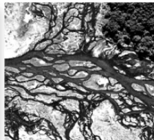
c. Random, sinuous braided stream pattern on a sandy soil at Pen Branch, SC.
